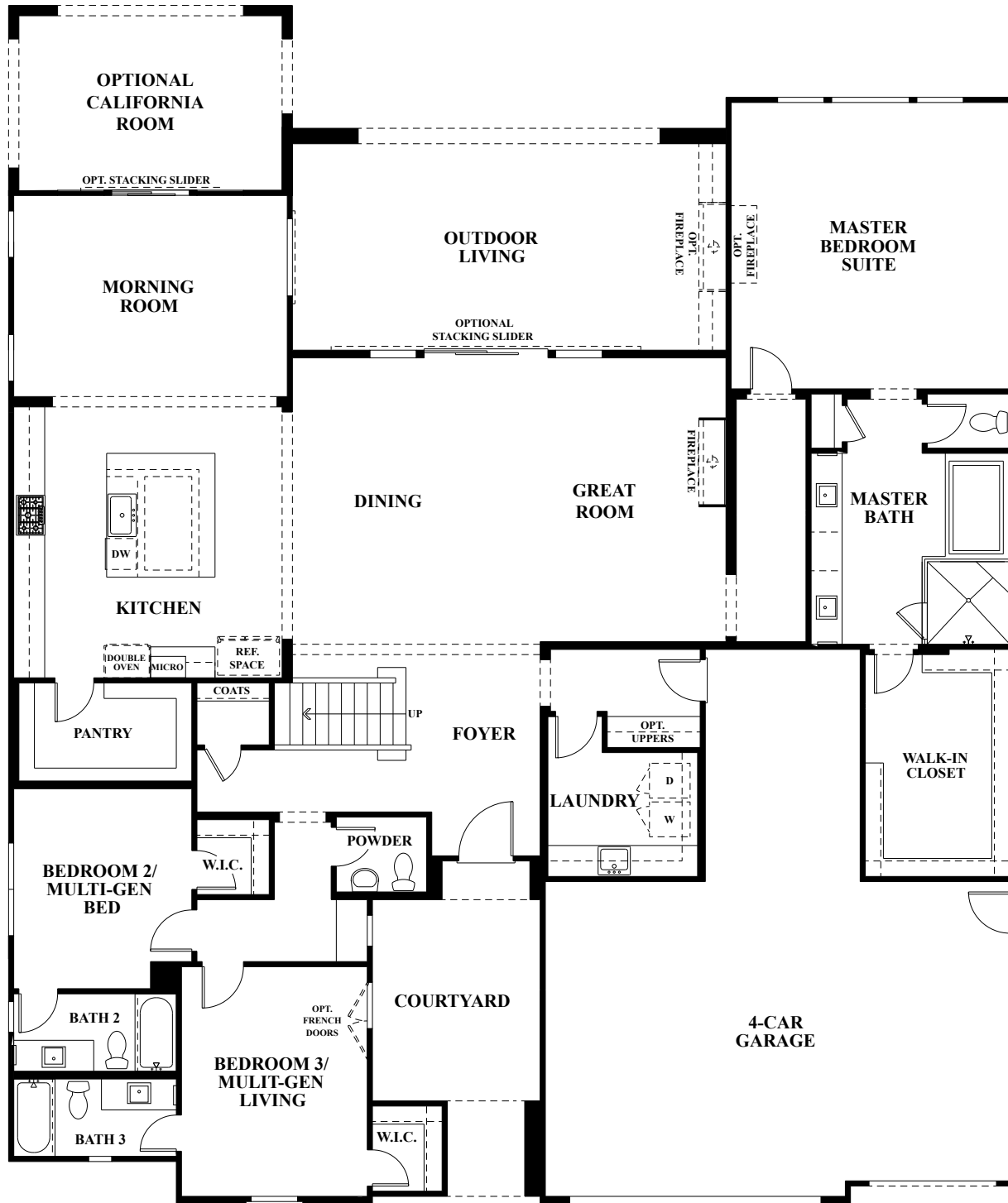
FIRST FLOOR
