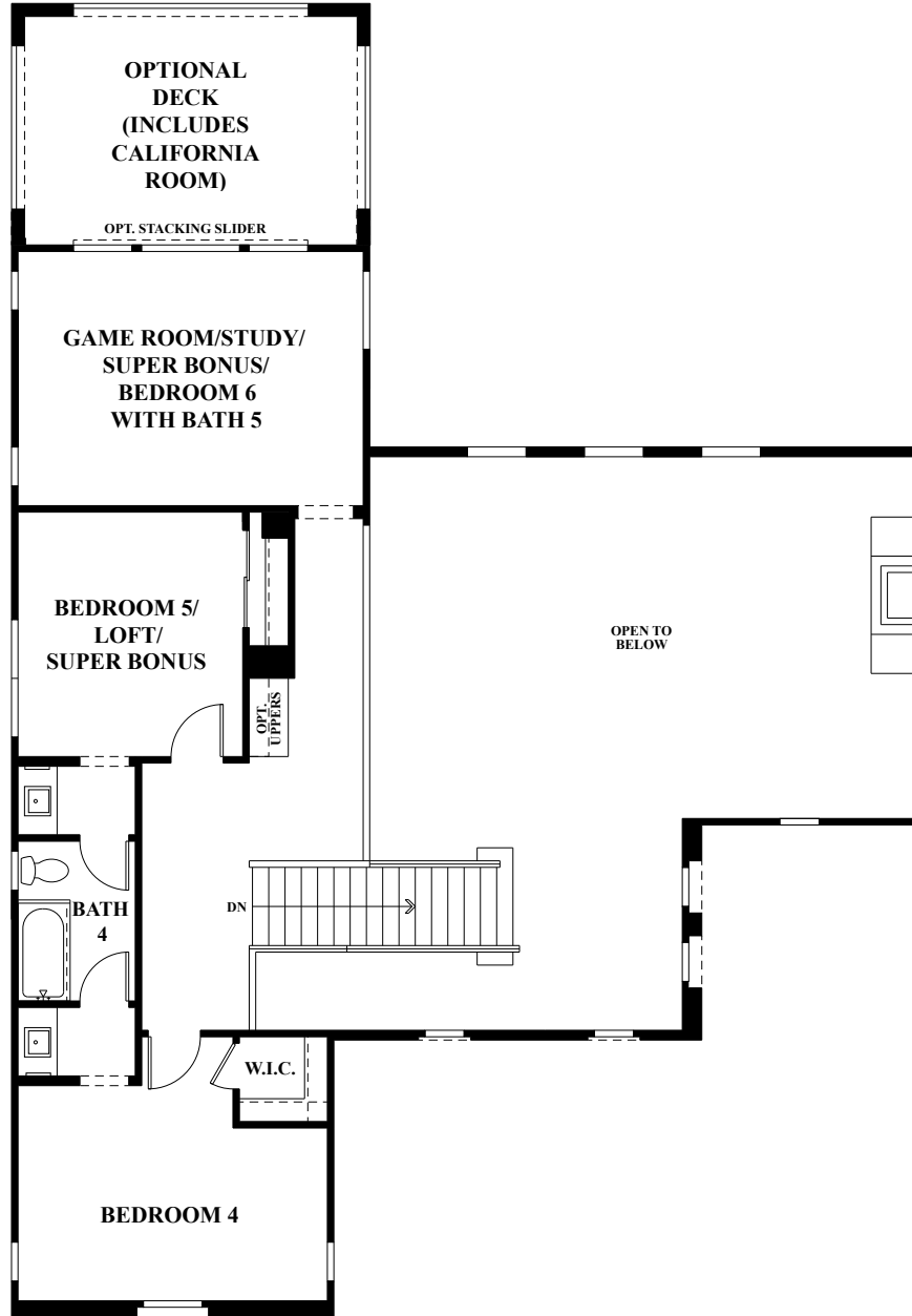
SECOND FLOOR
