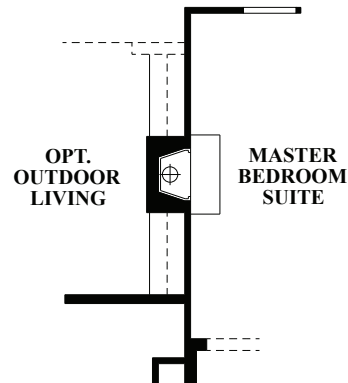
OPTIONAL FIREPLACE AT MASTER BEDROOM SUITE
